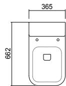
Cassetta 31CM
