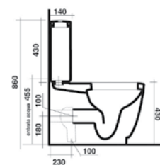
Cassetta 23CM
